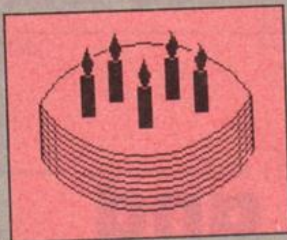
Listing 1
